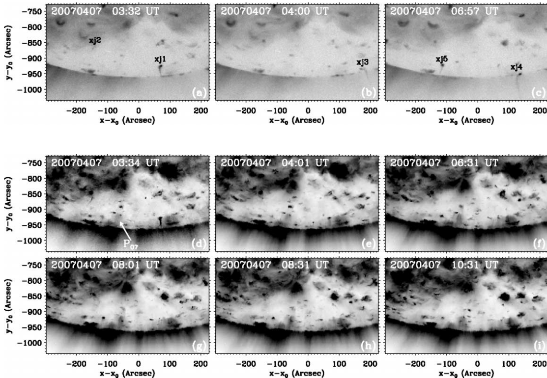
FIG. 3.— Top: Hinode /XRT snapshots of the southern polar coronal hole recorded on 2007 April 7 showing several X-ray jet events. X-ray jets are labeled by xj_i ( i = 1, \dots, 5 ) according to their time of appearance. Middle and bottom: 171 Å images from STEREO /SECCHI/EUVI “A” of the southern polar hole of the same day. Polar plume haze clearly rises from the same locations as X-ray and EUV jets with a time delay ranging from minutes to hours. A number of short-lived, jetlike events also occur at the base of polar plumes.
