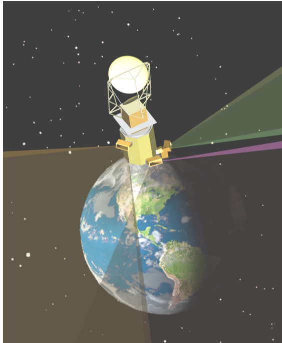
Figure 5. Schematic of SMEI in orbit. The spacecraft orbit is nearly circular at 840 km above the surface of the Earth with an inclination of 98^\circ relative to the equatorial plane. SMEI looks outward from the Earth over an \sim 180^\circ range of sky from three baffled cameras. The SMEI cameras and their fields of view as depicted are directed approximately 30^\circ above the local horizontal to avoid both light from the Earth and sunlight reflecting from the rotating Windsat antenna (see also Figure 2).
