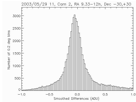
Figure 8. Histogram of a 40^\circ by 60^\circ portion of the sky map in Figure 7a from right ascension 9hr 20m and declination -30 respectively (to the solar southeast centered on an elongation 90^\circ from the Sun). The response on the ordinate is in Analog to Digital Units (ADU). Ground-based and SMEI on-orbit “G-type” stellar subtractions give a preliminary calibration of this histogram of 1 \text{ S10} \approx 0.55 \text{ ADU} , and thus the mean square difference for the portion of the sky map that makes up the histogram is \sim 0.2 \text{ S10} .
