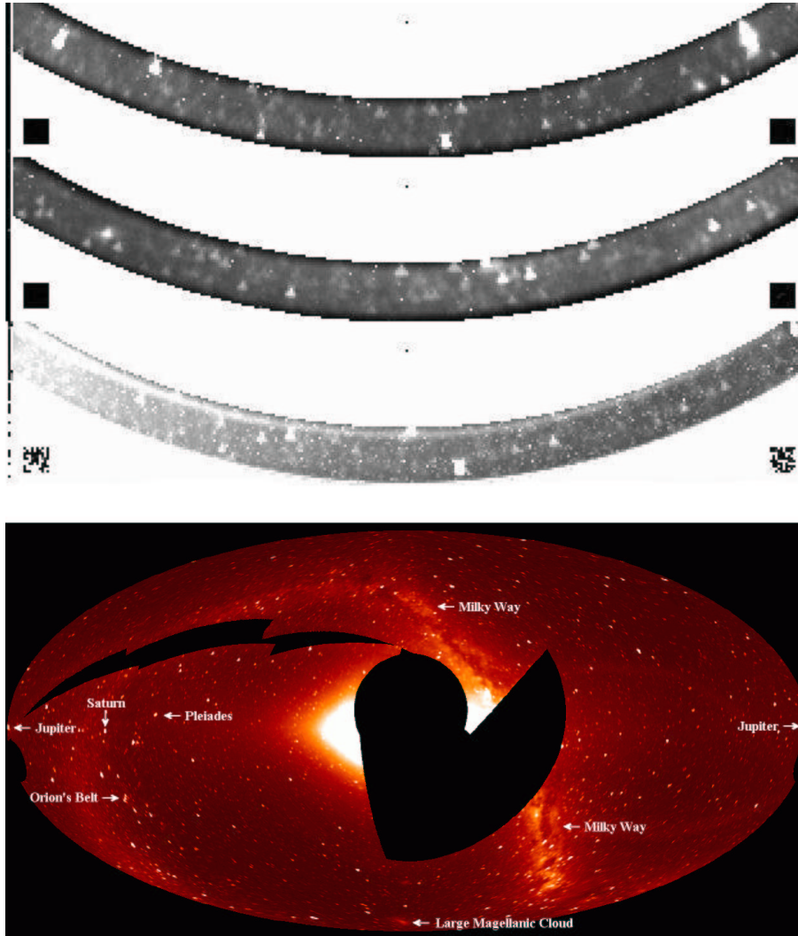
Figure 6. a) SMEI 3^\circ \times 60^\circ data frames from each of the three cameras arranged in order from top to bottom, the one viewing farthest to the one viewing nearest the Sun. The Sun is located towards the left in each data frame. b) A full orbit's worth of frames are registered onto a high resolution sky map and together build a composite view of the sky over that orbit that can be projected as a sky map (here shown as a full-sky Hammer-Aitoff projection). Various bright features are labeled on the map. Blank areas are regions that were excluded from the composite view either because they were not accessible to the cameras during the orbit, were too close to the Sun and thus too bright, or were contaminated by Earth radiation-belt particle enhancements (the slash across the upper left of the sky map).
