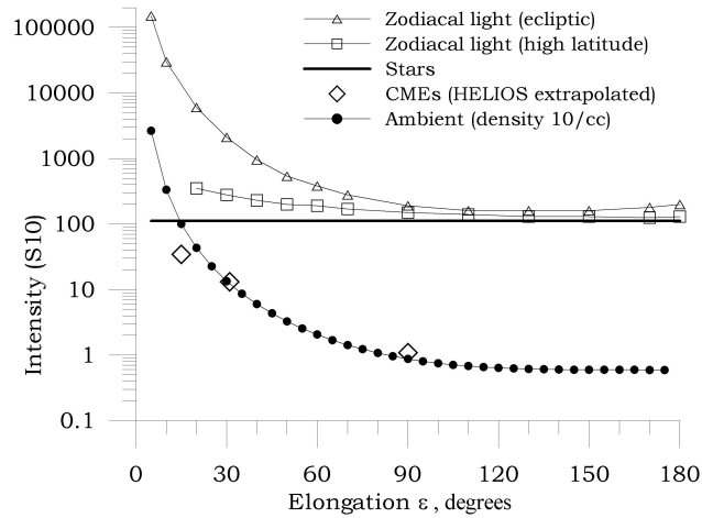
Figure 3. Surface brightness versus solar elongation for zodiacal and star light ( Allen's Astrophysical Quantities , 2000), and of expected CME brightness extrapolated from Helios measurements. A calculation of an ambient medium having a density of 10 \text{ e}^- \text{ cm}^{-3} at 1 AU and an inverse-square density dropoff with solar distance is also shown.
