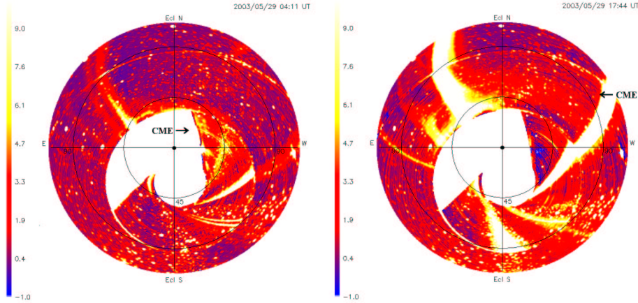
Figure 7. Shown are “fisheye” 102-minute composite sky maps from two orbits of data differenced from an 8-orbit average for SMEI Cameras 1 and 2 data with CCD pixels binned using normal science mode operation ( 4\times4 ) and for SMEI Camera 3 data binned 2\times2 . The differences show a CME (arrow) that was observed on 28 May 2003 to surround the Sun in the LASCO data. The brightness scale is in ADU. The blank area in the middle of the map is the location that cannot be accessed at this time of the year where Camera 3 looks too close to the Sun. These data have been averaged into 1^\circ bins using a Gaussian filter that extends circularly in spherical angle from each location on the map. Circles on the map are Sun-centered at 45^\circ and 90^\circ elongation; ecliptic north is at the top. The beginning time of the data that produces the sky map is indicated to the upper right of the map, and for this display proceeds clockwise around map center from the southernmost point of the map. The oblong points scattered throughout the map are mostly variable stars that have changed brightness relative to the subtracted minimum. The techniques used to provide these sky maps are outlined in Appendix 1. a) The outer edge of the CME is at about 45^\circ elongation due north and encircles the Sun from northwest to south reaching \sim 60^\circ elongation due west. b) The CME has progressed farther and portions of its bright portions have reached beyond 90^\circ (at least 1 AU) to the northeast and south completely encircling the Sun and raising the general background level over nearly the entire sky. The blank approximately radial region to the solar northeast in this map is a bright band of auroral light where SMEI passes through the Earth’s northern auroral oval. The blank radial region to the solar northwest is a location where energetic charged particles were too numerous to allow the desired photometric performance as SMEI passed through the South Atlantic Anomaly.
