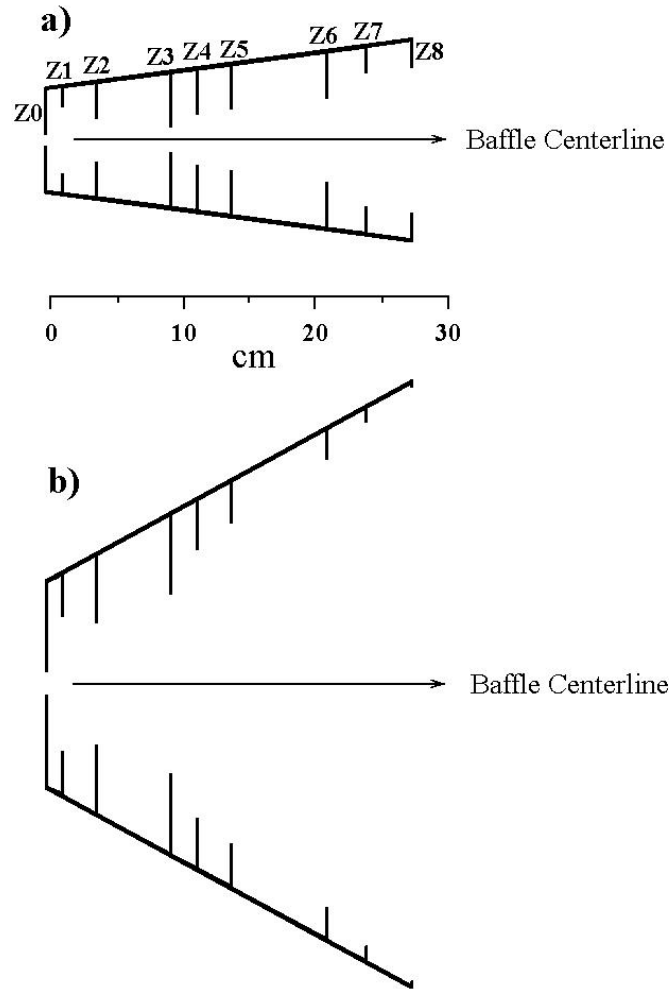
Figure 4. Schematic of SMEI baffle. The scale is in centimeters. Apertures are numbered Z0 to Z8 in advancing distance towards incident light along the baffle centerline. a) Narrow dimension. b) Wide dimension.
