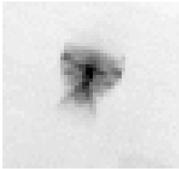
Figure 9. Shown is a typical unresolved SMEI stellar image ( \beta Draco, M_v = 2.79 ). The image shape is produced by the fast ( \sim f/1 focal ratio) SMEI optics which spreads the light from a point source as uniformly as possible over \sim 200 CCD pixels. The scan direction for the SMEI instrument is approximately from top to bottom in this image.
